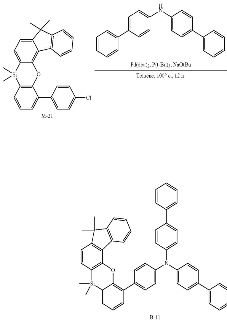
[Reaction Scheme 33]
